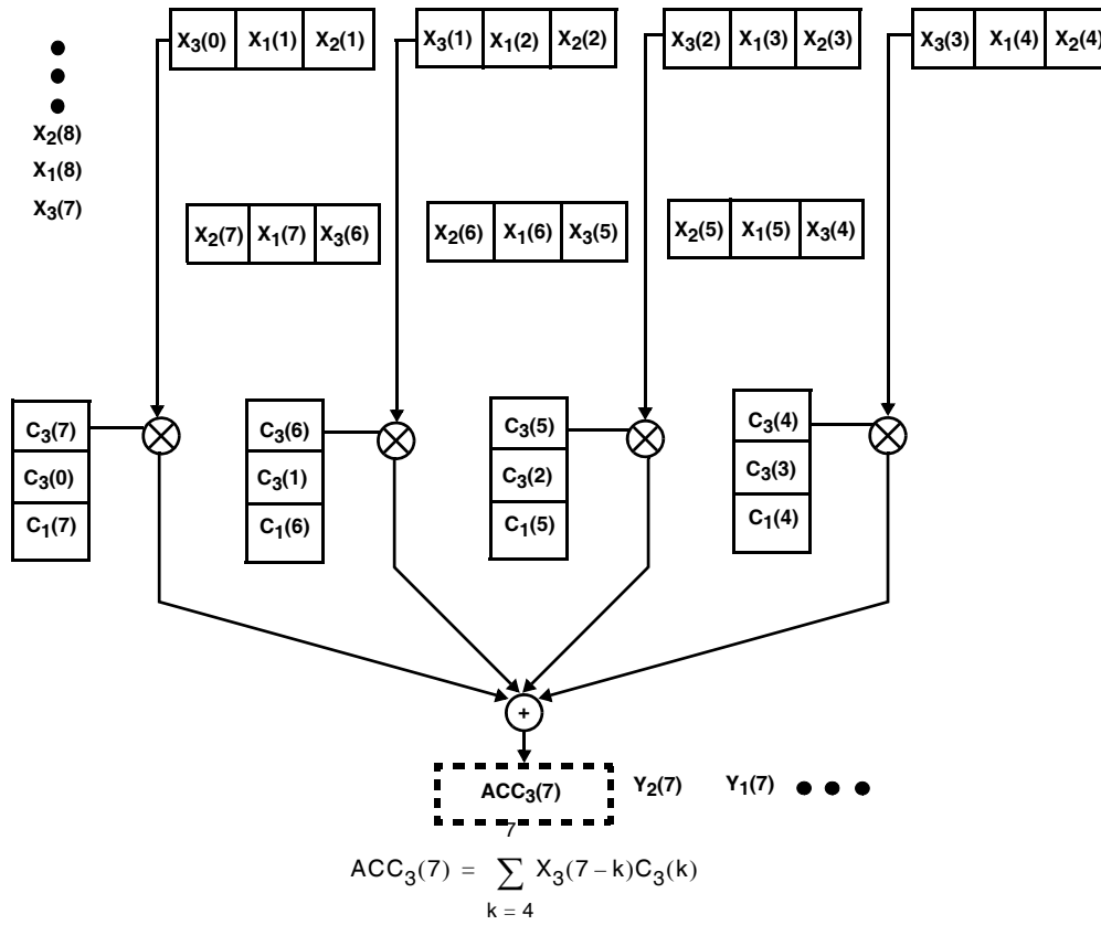
FIGURE 6E. DOUBLE-CLOCKED ASYMMETRIC MULTI-CHANNEL DATA FLOW DIAGRAM STEP 5
