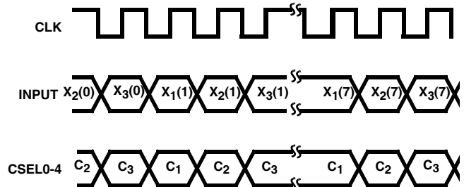
FIGURE 2C. SYMMETRIC MULTI-CHANNEL DATA FLOW DIAGRAM STEP 3
